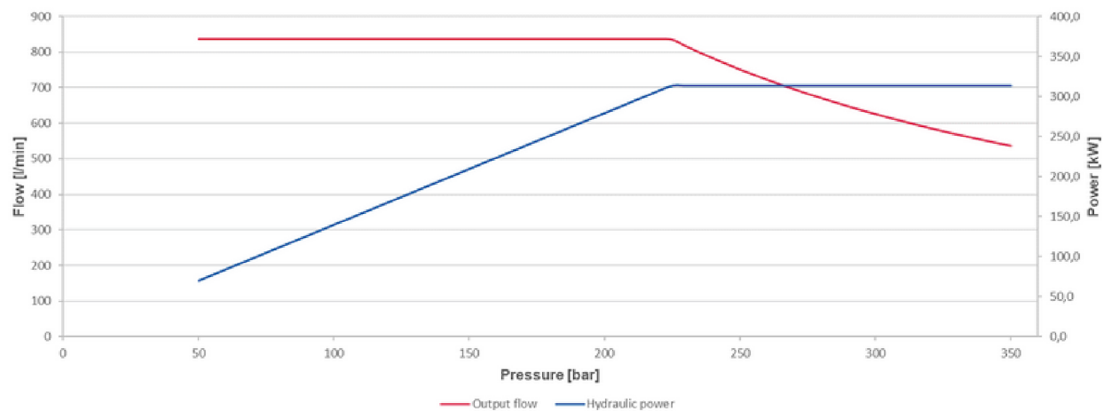
HydrauPack 360E Battery @370 [kW] | Peak Shaving Supply | 38 [min]
